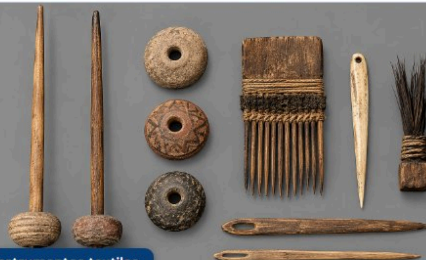
Instrumentos textiles
